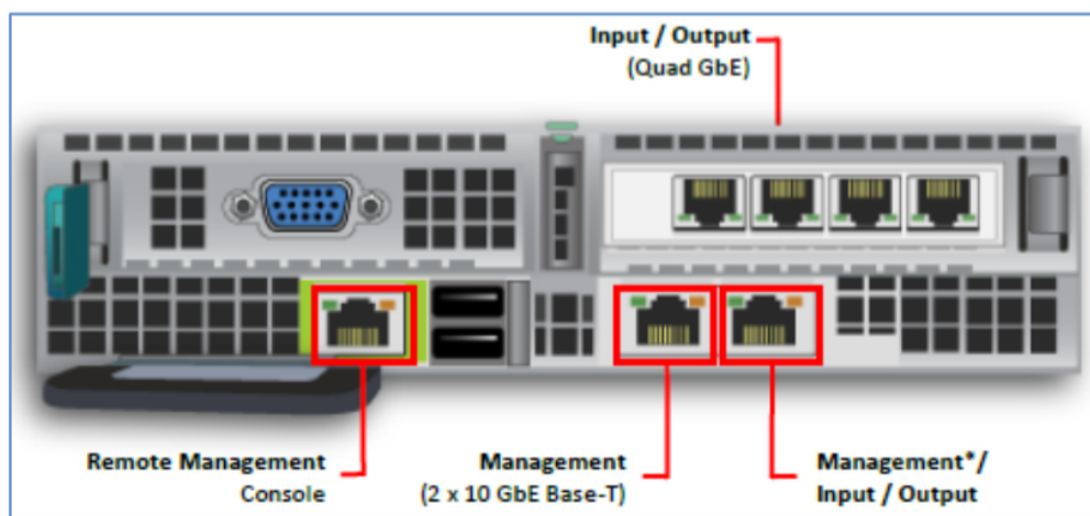
Figure 2: Network interfaces Connection on G8 2000 Series .
