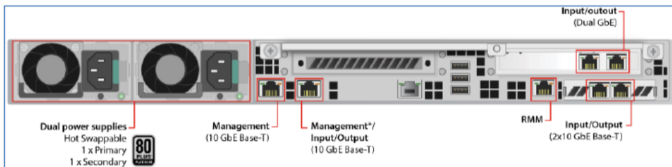
Figure 1: Network interfaces Connection on G8 1000 Series .
